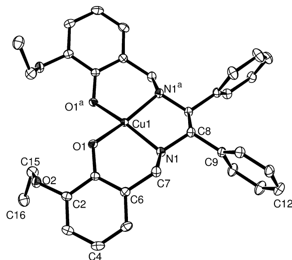
Fig. 1 Molecular structure of one of the two independent molecules (molecule A) of [Cu(2)] with ellipsoids plotted at the 50% probability level, and H atoms omitted. Selected bond parameters for molecule A: Cu1–N1 = 2.023(2), Cu1–O1 = 1.917(1) Å; N1–Cu1–O1 = 94.24(5)°, N1–Cu1–N1 a = 84.01(8)°, O1–Cu1–O1 a = 93.57(6)°, N1–Cu1–O1 a = 160.69(5)°. For molecule B: Cu2–N2 = 2.024(1), Cu2–O3 = 1.923(1) Å; N2–Cu2–O3 = 93.55(5)°, N2–Cu2–N2 b = 85.23(8)°, O3–Cu2–O3 b = 89.80(6)°, O3 b –Cu2–N2 = 168.69(5)°. Symmetry codes: a = 1 – x , y , 1 – z ; b = 1 – x , y , – z .
