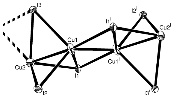
Fig. 2 Part of one polymeric chain in [iPr_2EtNH]_n[Cu_2I_3]_n with ellipsoids plotted at the 50% probability level. Symmetry codes: i = 1 - x, 1 - y, 1 - z ; ii = 2 - x, 1 - y, 1 - z . Selected bond distances: I1-Cu1^i = 2.5382(3) , I1-Cu1 = 2.7280(3) , I1-Cu2 = 2.7903(3) , I2-Cu1 = 2.6736(3) , I2-Cu2 = 2.6764(3) , I3-Cu2^{ii} = 2.5422(3) , I3-Cu1 = 2.7841(3) , I3-Cu2 = 2.7328(3) , Cu1-Cu1^i = 2.6276(5) , Cu1-Cu2 = 2.4900(3) , Cu2-Cu2^{ii} = 2.6378(5) Å.
