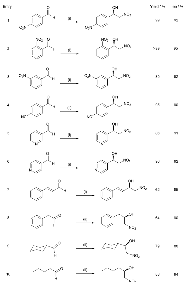
Fig. 3 Results of the enantioselective Henry reaction of nitromethane and selected aldehydes under optimized reaction conditions. (i) H_22 (5 mol%), CuI (10 mol%), THF, 273 K, 12 h. (ii) H_22 (5 mol%), CuI (10 mol%), THF, 295 K, 72 h.
